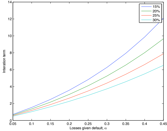
Figure 2: The indirect effect of a shock to losses given default. This figure plots the absolute size of the interaction term \frac{dFDC}{dV_B} \cdot \frac{dV_B}{d\alpha} in equation (4) as a function of the level of losses given default ( \alpha ) for various levels of asset volatility ( \sigma ). We set the initial asset value to 100, the risk-free rate to 5%, the average debt maturity to T = \frac{10}{2} , the cash payout rate to 6%, the corporate tax rate to 15%, and the aggregate debt service to C = 5 , P = 50 .
