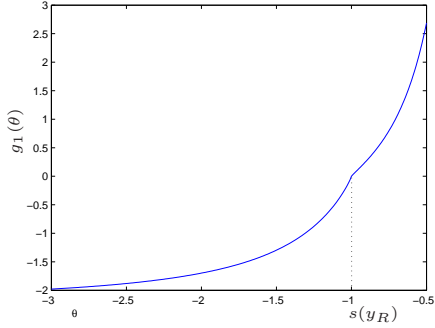
(a) (I). \beta = -0.5 , \alpha_1 = 0.9 , s(y_R) = -1 . Wait for all values of \theta and equivalently, for all prices y .
