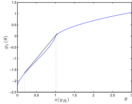
(d) (III). \beta = 1.5 , \alpha_1 = 0.7 , s(y_R) = 1 . Waits for \theta \in (\bar{\theta}_l^{(1)} = 0.1723, \bar{\theta}_u^{(1)} = 1.0105) and stops otherwise. Equivalently, waits for y \in (\bar{y}_l^{(1)} = 0.31, \bar{y}_u^{(1)} = 1.007) .
