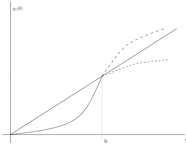
Figure 8: The solid curve and its two possible dashed continuations give a stylized representation of possible functions g_1(\theta) as a function of scaled price \theta , where \theta = s(y) . The function g_1(\theta) represents the value of the game to the agent if he sells immediately. The point B marks the break-even point. To decide whether the agent stops at or to the right of point B involves comparing the slope of the chord from the origin to B with the slope of the function to the right of B.
