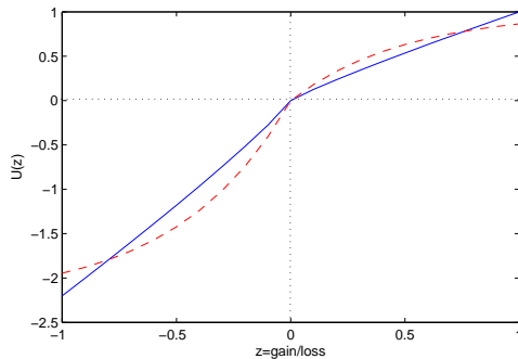
Figure 1: The Tversky and Kahneman (1992) S -shaped function U(z) given in (1) with loss aversion \lambda = 2.25 and \alpha_1 = \alpha_2 = 0.88 is given by the solid line. The piecewise exponential S -shaped function U(z) given in (2) with \phi_1 = 1, \phi_2 = 2.25, \gamma_1 = \gamma_2 = 2 is given by the dashed line.
