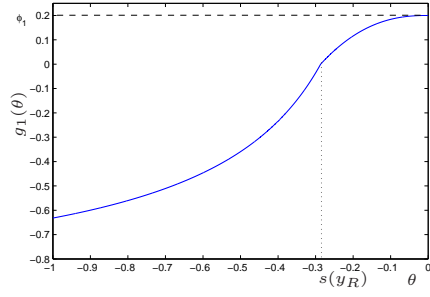
(b) (I). \mu = 0.1 , s(y_R) = -0.2865 . Wait at all values of \theta ; equivalently at all prices y .
