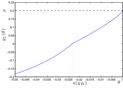
(a) (I). \mu = 0.3 , s(y_R) = -0.0235 . Wait at all values of \theta ; equivalently at all prices y .
