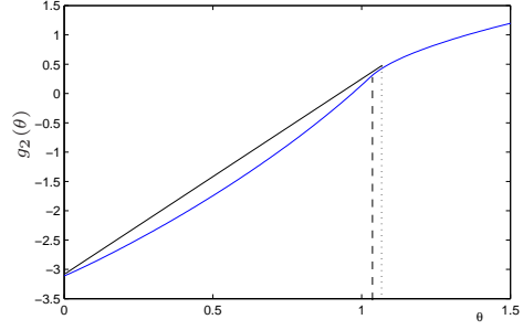
(b) (II). \beta = 0.75 , \alpha_1 = 0.5 < \beta , \lambda = 2.2 , \hat{\theta}_u^{(2)} = 1.0302 , \bar{\theta}_u^{(2)} = 1.06 , s(y_R) = 1 and \bar{y}_u^{(2)} = 1.08 .
