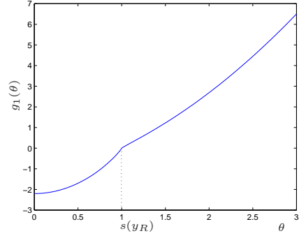
(b) (I). \beta = 0.5 , \alpha_1 = 0.9 , s(y_R) = 1 . Waits for all values of \theta and equivalently, for all prices y .
