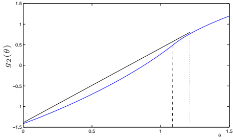
(a) (II). \beta = 0.75 , \alpha_1 = 0.5 , \lambda = 1 , \hat{\theta}_u^{(2)} = 1.1 , \bar{\theta}_u^{(2)} = 1.23 , s(y_R) = 1 and \bar{y}_u^{(2)} = 1.32 .
