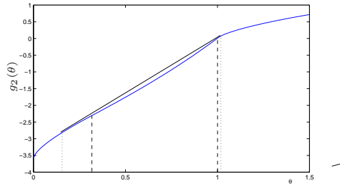
(d) (III). \beta = 1.5 , \alpha_1 = 0.7 , \lambda = 2.2 , \hat{\theta}_l^{(2)} = 0.3252 , \hat{\theta}_u^{(2)} = 1.0052 , \bar{\theta}_l^{(2)} = 0.17 , \bar{\theta}_u^{(2)} = 1.01 , and s(y_R) = 1 . Also \bar{y}_l^{(2)} = 0.31 , \bar{y}_u^{(2)} = 1.007 .
