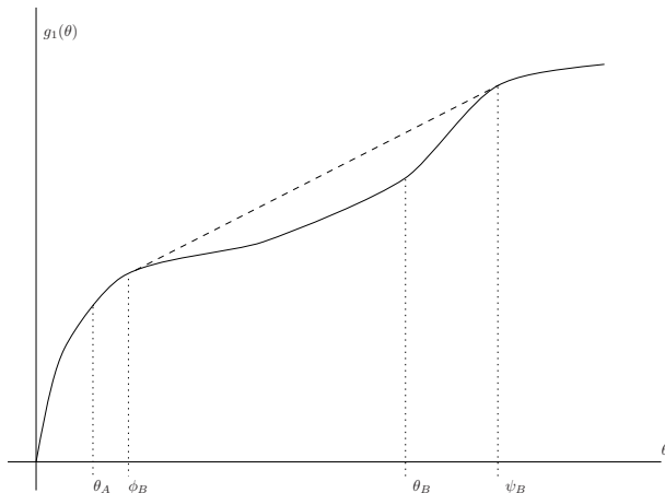
Figure 2: Stylized representation of the function g_1(\theta) as a function of transformed price \theta , where \theta = s(y) . The function g_1(\theta) represents the value of the game to the agent if she sells immediately. The smallest concave majorant \bar{g}_1(\theta) is formed by taking the straight dashed line for \theta \in (\phi_B, \psi_B) and the function g_1 itself for \theta \leq \phi_B and \theta \geq \psi_B .
