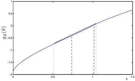
(c) (III). \beta = 1.5 , \alpha_1 = 0.88 , \lambda = 1 , \hat{\theta}_l^{(2)} = 0.6971 , \hat{\theta}_u^{(2)} = 1.0252 , \bar{\theta}_l^{(2)} = 0.52 , \bar{\theta}_u^{(2)} = 1.05 , s(y_R) = 1 . Also \bar{y}_l^{(2)} = 0.65 , \bar{y}_u^{(2)} = 1.03 .
