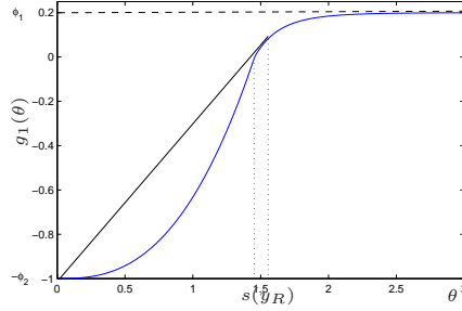
(c) (II). \mu = -0.03 , s(y_R) = 1.455 . Stop for \theta > 1.54 (where s(y_R) < 1.54 ); or equivalently, for prices y > s^{-1}(1.54) = 1.15 > y_R = 1 .
