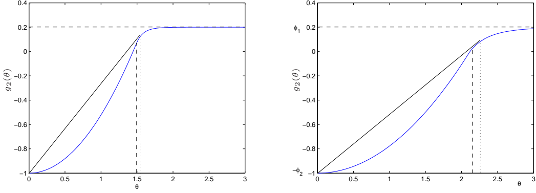
(a) (II). \mu = -0.03 , \sigma = 0.4 , \hat{\theta}_u^{(2)} = 1.4923 , \bar{\theta}_u^{(2)} = 1.55 , s(y_R) = 1.455 and \bar{y}_u^{(2)} = 1.173 . (b) (III). \mu = -0.06 , \sigma = 0.4 , \hat{\theta}_u^{(2)} = 2.117 , \bar{\theta}_u^{(2)} = 2.23 , s(y_R - x) = 2.117 and \bar{y}_u^{(2)} = 1.067 .
