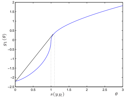
(c) (II). \beta = 0.75 , \alpha_1 = 0.5 , s(y_R) = 1 . Stops for \theta \geq \bar{\theta}_u^{(1)} = 1.06 or equivalently for y \geq \bar{y}_u^{(1)} = 1.08 .
